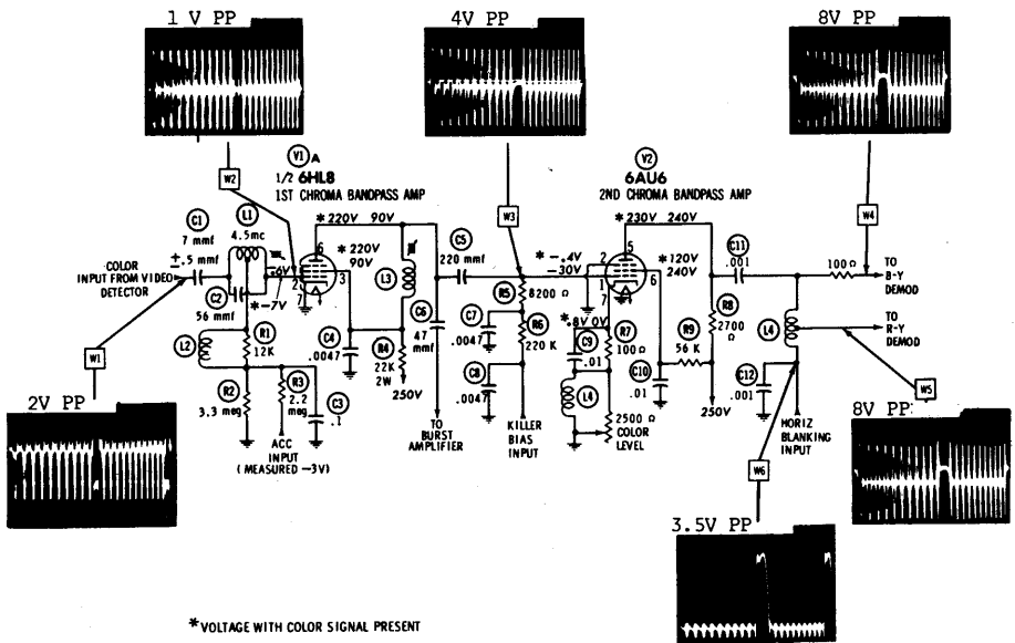
Fig. 3 - Two-stage Zenith Bandpass amplifier
