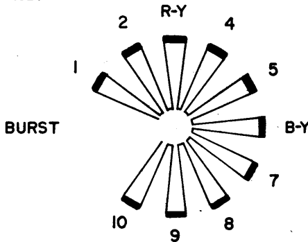
Fig. 8 - Ideal vector display on Vectorscope
