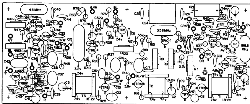
Fig. 12 - P.C. Board layout
