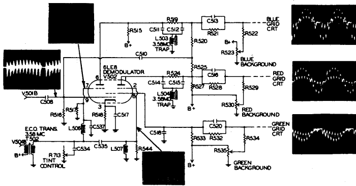
Fig. 6 - High level demodulator used in Color TV
