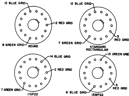
Fig. 1 - Rear View of Color tube bases
